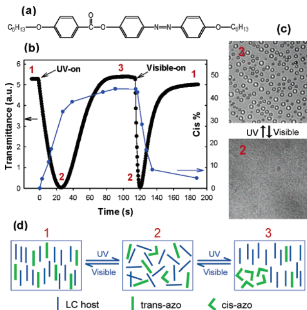
Figure 1. (a) Chemical structure of the liquid crystalline azo dopant. (b) Change in transmittance of BL006/dopant (15%) exposed to UV ( 6.5 mW \text{cm}^{-2} ) and visible light ( 4.5 mW \text{cm}^{-2} ), and variation of the amount of cis azobenzene in the mixture. (c) Photomicrographs of the mixture in states 2 and 3 marked in (b) (image area: 50 \times 50 \mu\text{m}^2 ). (d) Schematic illustration of the reversible and interconvertible photochemical phase transition and photochemical phase separation.
